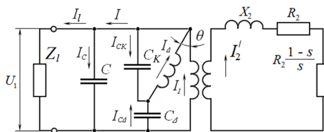
Figure 5. Wiring diagram of CIG phases
