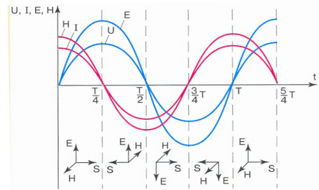
Fig. 6. Direction of the Poynting vector \vec{S} along the single-conductor line in the standing-wave regime: I , H – waves of the current and the magnetic field strength; V , E – waves of the voltage and the electric field strength.
