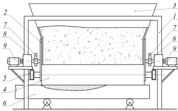
Fig. 5. Roller forming installation with the cam driving mechanism.
