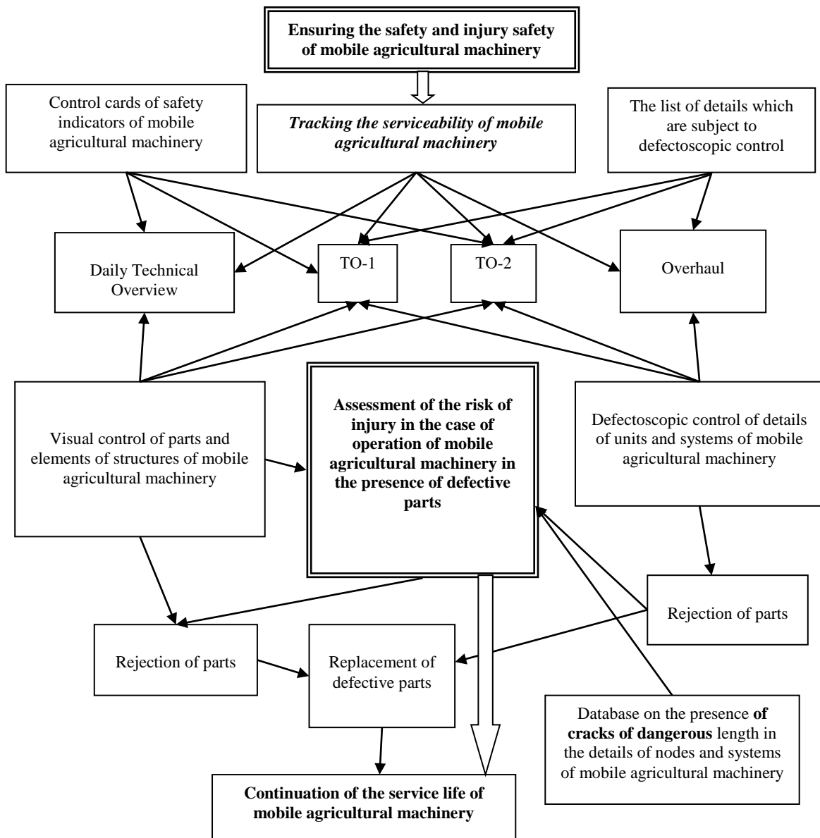
Fig. 5. Algorithm for assessing the serviceability of mobile agricultural machinery
