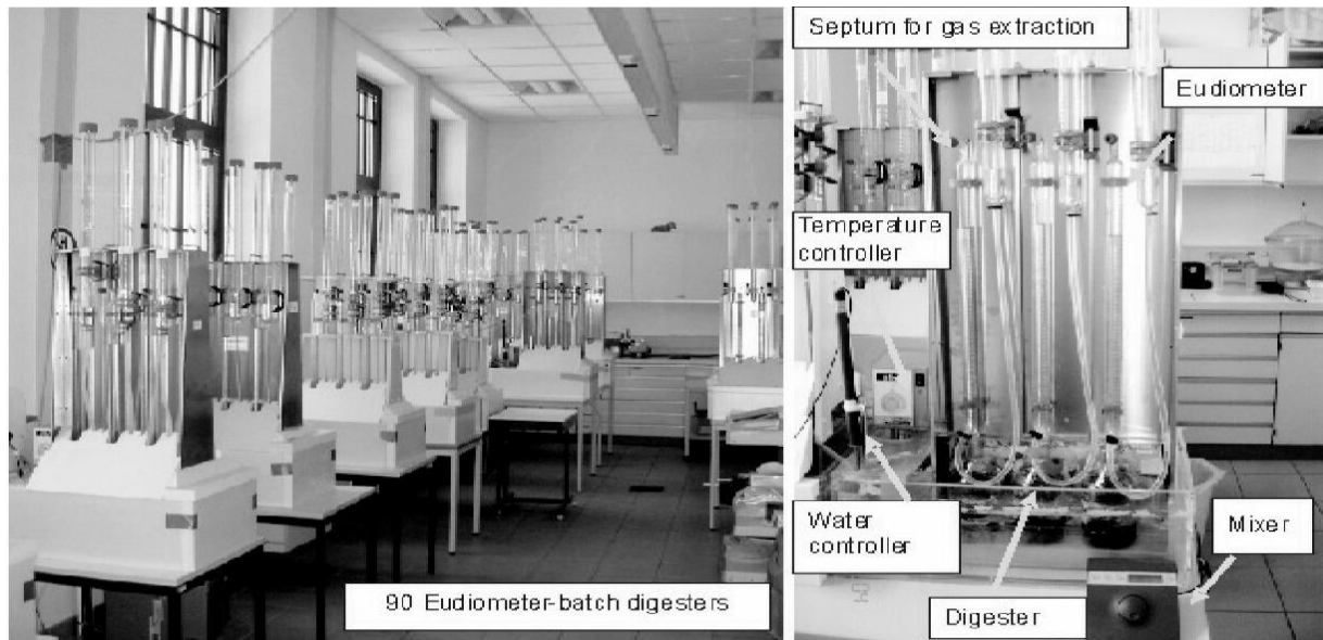
Fig. 1. Eudiometer-batch digester system.
