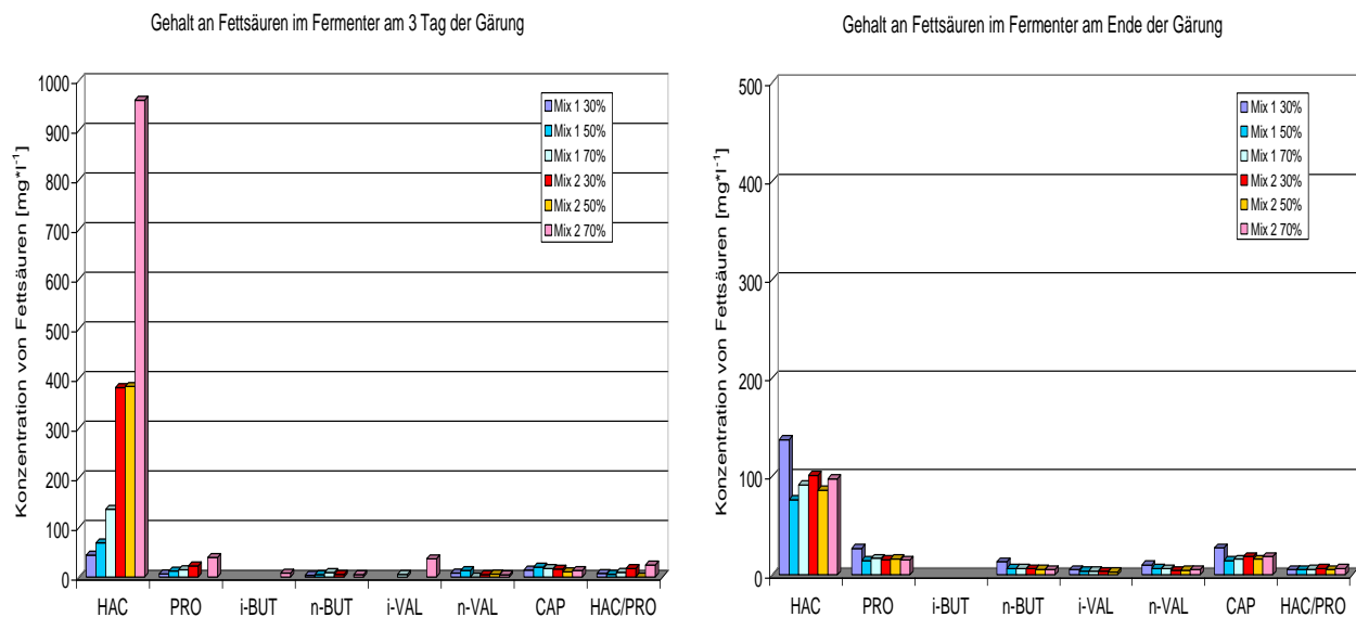
Fig. 2. Concentration of fatty acids in the fermenters to begin and to the end of digestion.
